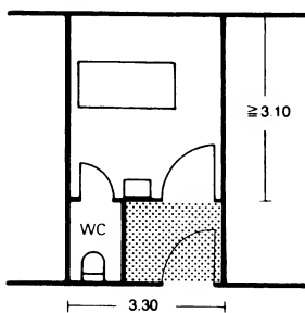
④ Single-bed room with lobby
